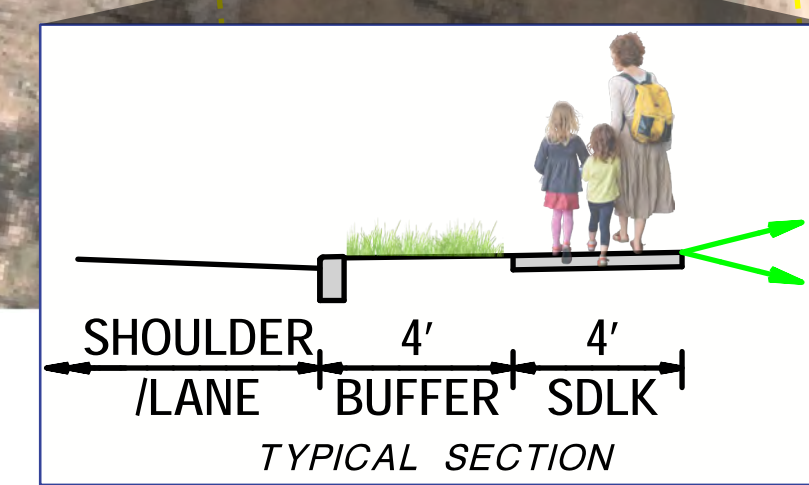
TYPICAL SECTION
