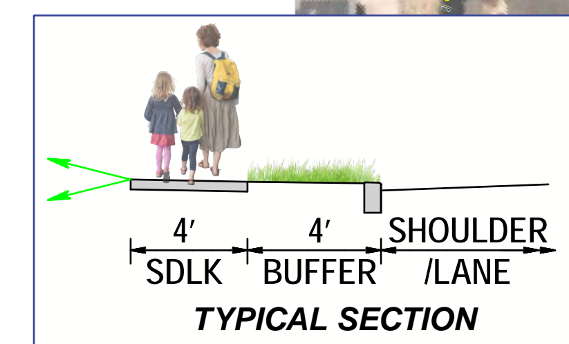
TYPICAL SECTION
